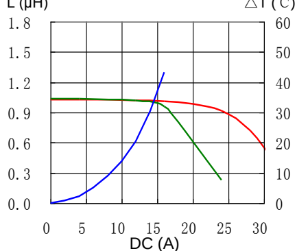
4. CDRH127/LDNP-4R6NC
