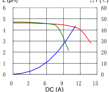
7. CDRH127/LDNP-100MC
