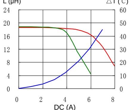
10. CDRH127/LDNP-180MC
