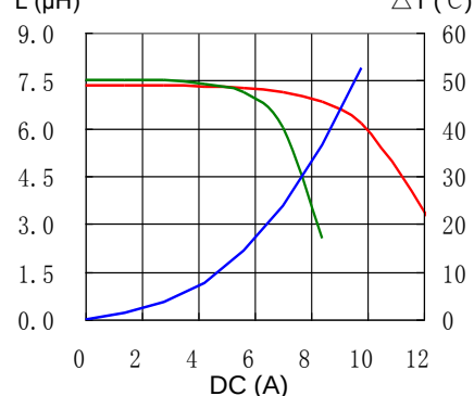
9. CDRH127/LDNP-150MC
