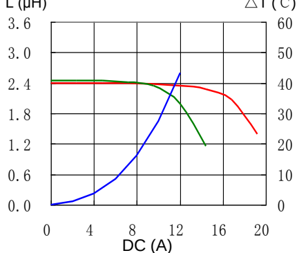
5. CDRH127/LDNP-5R8NC
