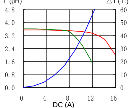
6. CDRH127/LDNP-7R4NC
