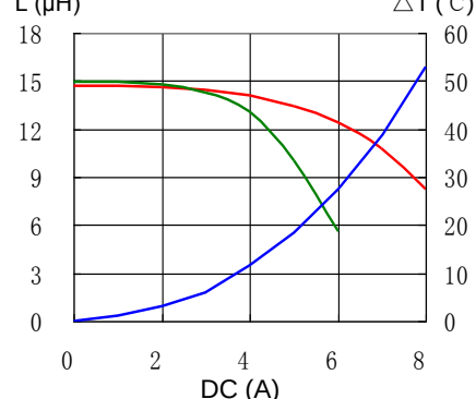
12. CDRH127/LDNP-270MC
