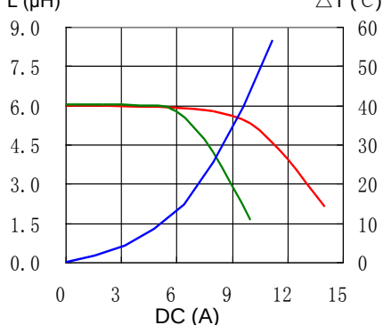
8. CDRH127/LDNP-120MC
